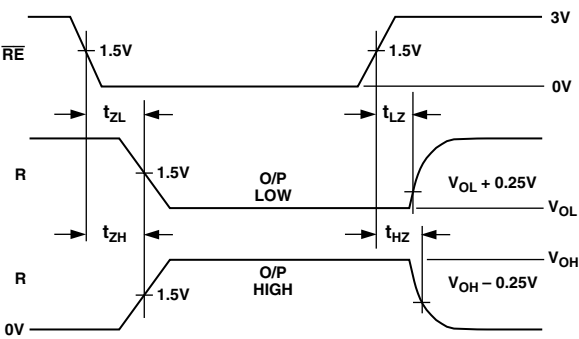
Figure 12. Receiver Enable/Disable Timing
