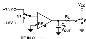
Figure 6. Receiver Enable/Disable Test Circuit
