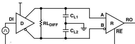
Figure 4. Driver/Receiver Propagation Delay Test Circuit
