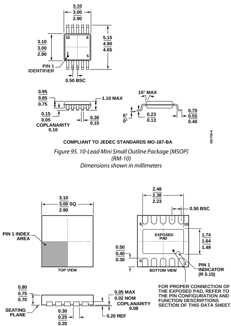
Figure 96. 10-Lead Lead Frame Chip Scale Package [LFCSP_WD] 3 mm × 3 mm Body, Very Thin, Dual Lead (CP-10-9)
