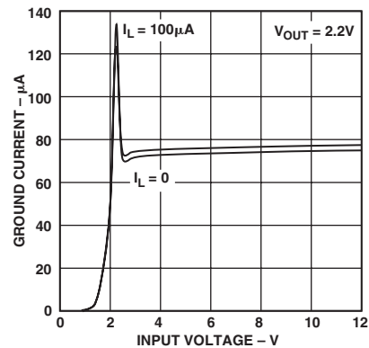
TPC 3. Ground Current vs. Supply Voltage
