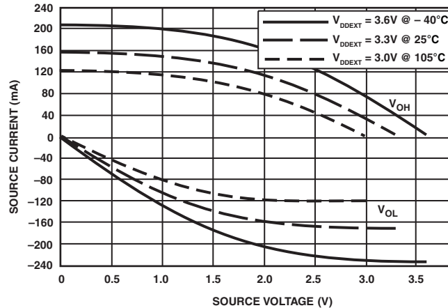
Figure 42. Driver Type B Current ( 3.3V_{DDEXT}/V_{DDMEM} )
