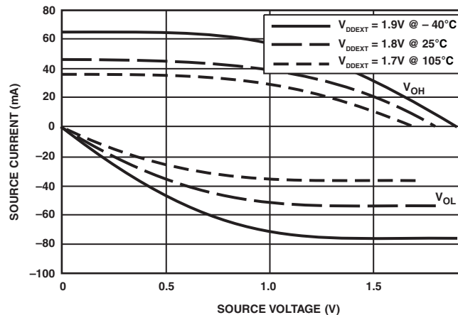
Figure 44. Driver Type B Current ( 1.8V_{DDEXT}/V_{DDMEM} )
