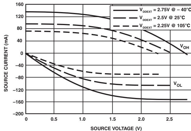
Figure 43. Driver Type B Current ( 2.5V_{DDEXT}/V_{DDMEM} )
