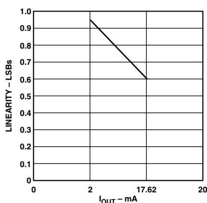
TPC 14. Linearity vs. I_{OUT}
