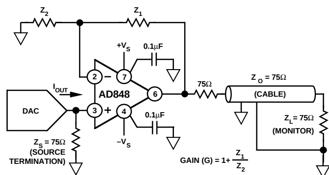
Figure 6. AD848 As an Output Buffer
