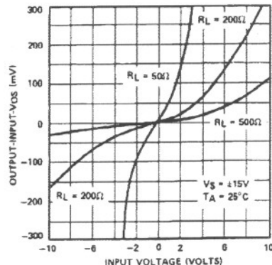
GAIN ERROR vs INPUT VOLTAGE
