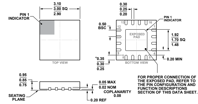
Figure 20. 16-Lead Lead Frame Chip Scale Package [LFCSP] 3 mm × 3 mm Body and 0.85 mm Package Height (CP-16-38)
