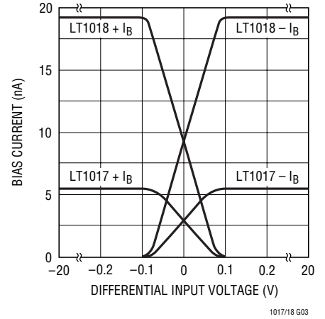
Bias Current vs Differential Input
