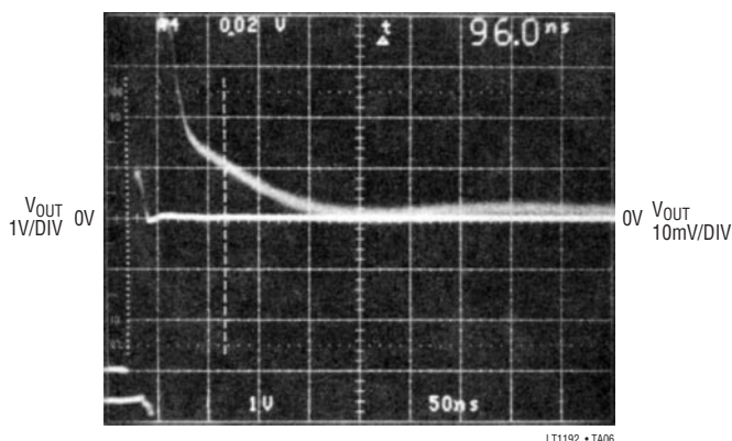
SETTLING TIME TO 10mV, A_V = 2 SUPPLY BYPASS CAPACITORS = 0.1μF + 4.7μF TANTALUM
