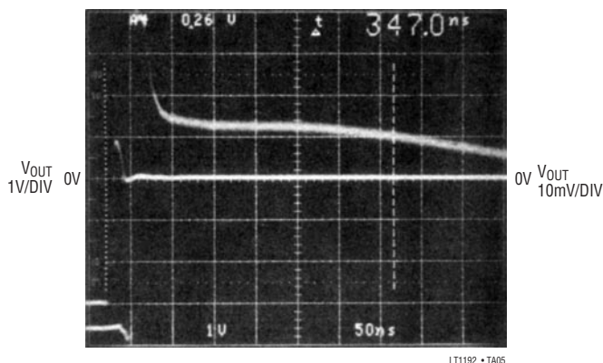
SETTLING TIME TO 10mV, A_V = 2 SUPPLY BYPASS CAPACITORS = 0.1μF
