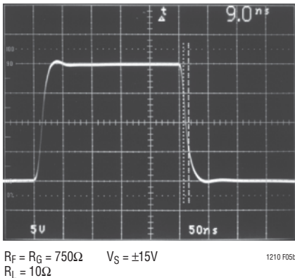
Figure 5b. Large-Signal Response, A_V = -1
