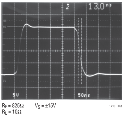
Figure 5a. Large-Signal Response, A_V = 1
