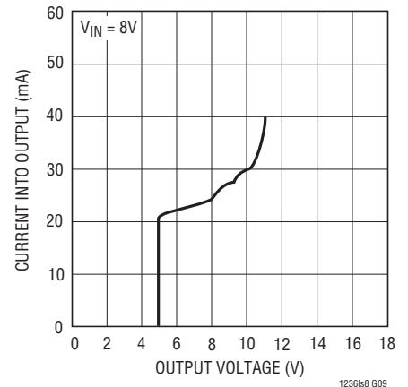
Sink Mode Current Limit
