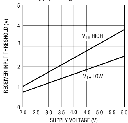
Receiver Input Thresholds vs Supply Voltage
