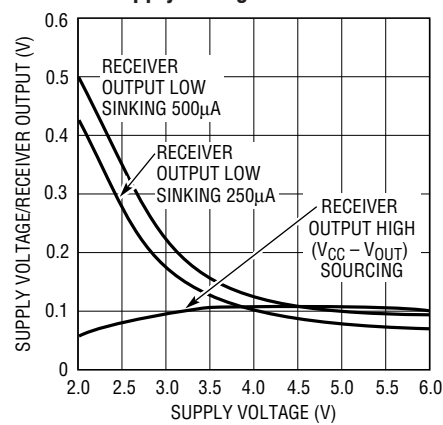
Receiver Output Voltage vs Supply Voltage
