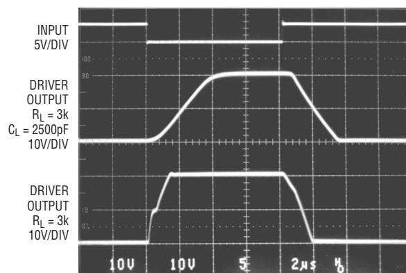
Driver Output Waveforms
