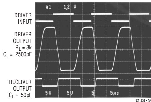
Output Waveforms
