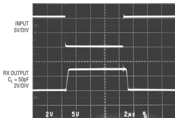
Receiver Output Waveforms
