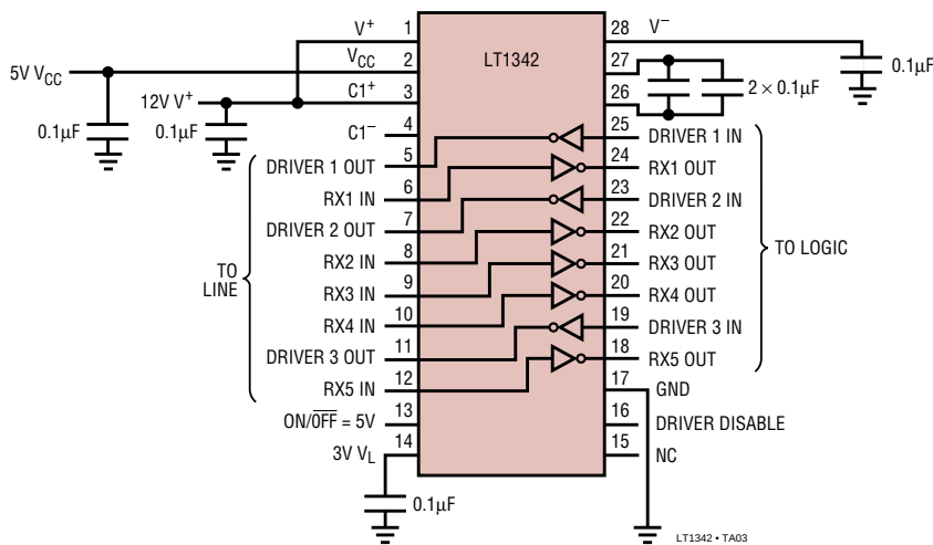
Operation Using 5V and 12V Power Supplies
