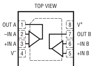
DD PACKAGE 8-LEAD (3mm \times 3mm) PLASTIC DFN T_{JMAX} = 150^\circ\text{C} , \theta_{JA} = 160^\circ\text{C/W} (NOTE 3) UNDERSIDE METAL CONNECTED TO V^- (PCB CONNECTION OPTIONAL)
