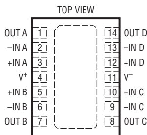
DE14 PACKAGE 14-LEAD (4mm \times 3mm) PLASTIC DFN T_{JMAX} = 150^\circ\text{C} , \theta_{JA} = 43^\circ\text{C/W} , \theta_{JC} = 4.3^\circ\text{C/W} EXPOSED PAD (PIN 15) IS V^- MUST BE SOLDERED TO PCB
