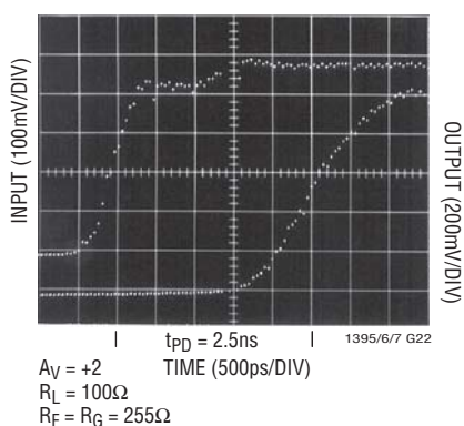
Propagation Delay
