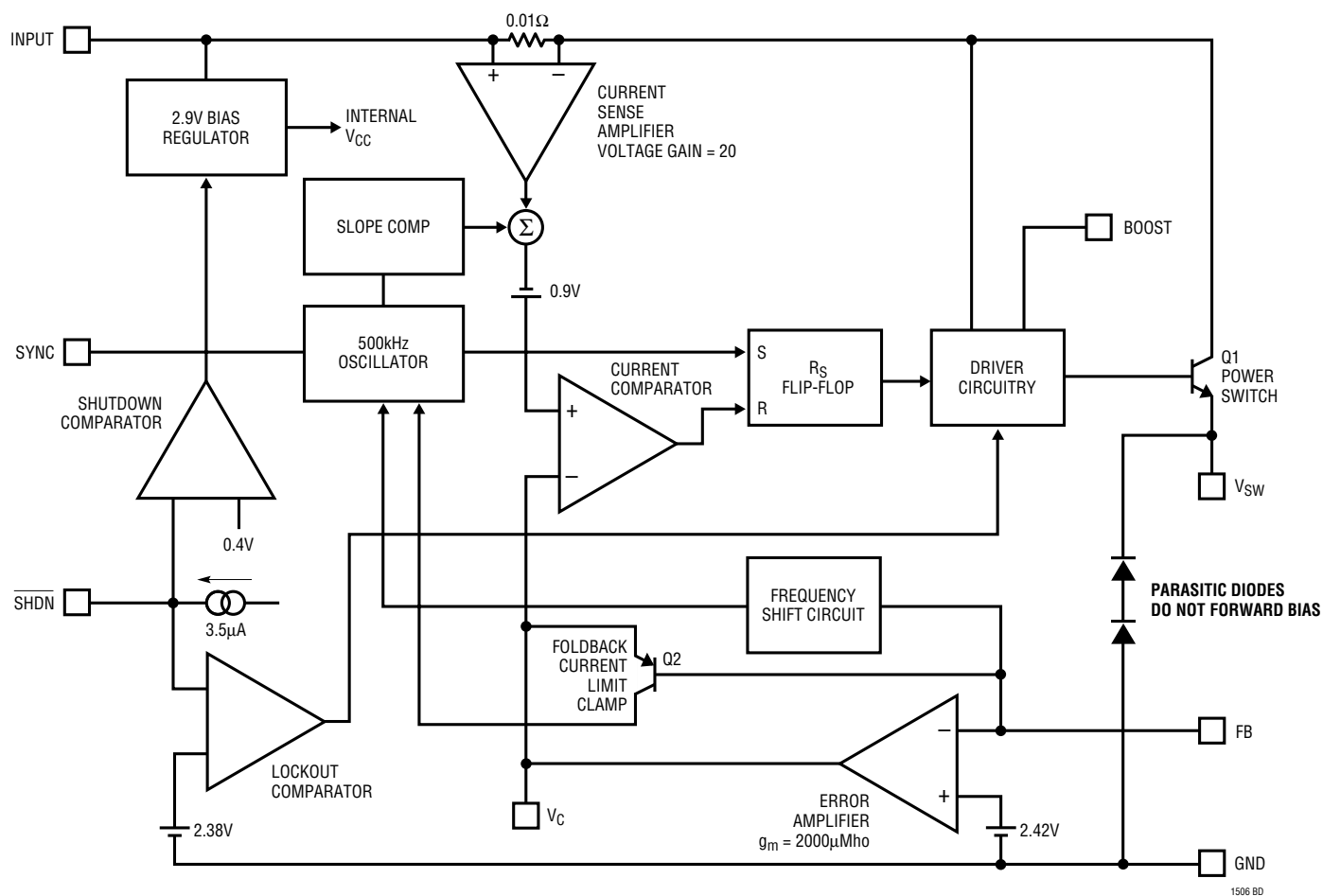
Figure 1. Block Diagram
