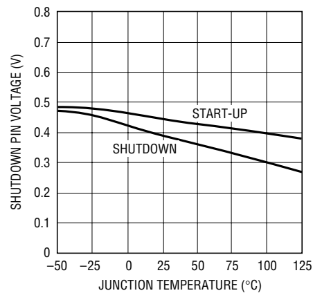
Shutdown Thresholds
