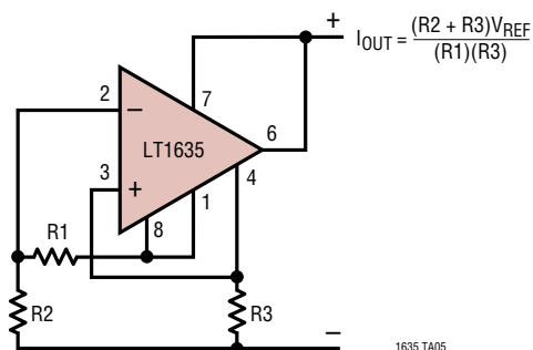
2-Terminal Current Regulator
