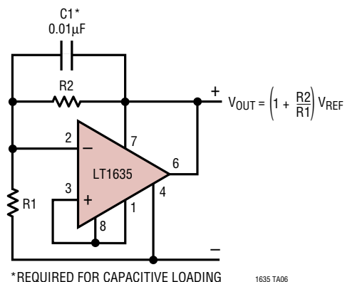
Shunt Regulator
