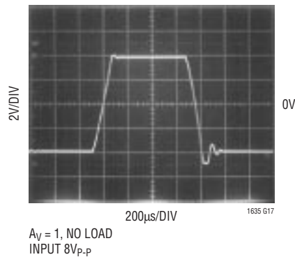
Large-Signal Transient Response V_S = \pm 5V
