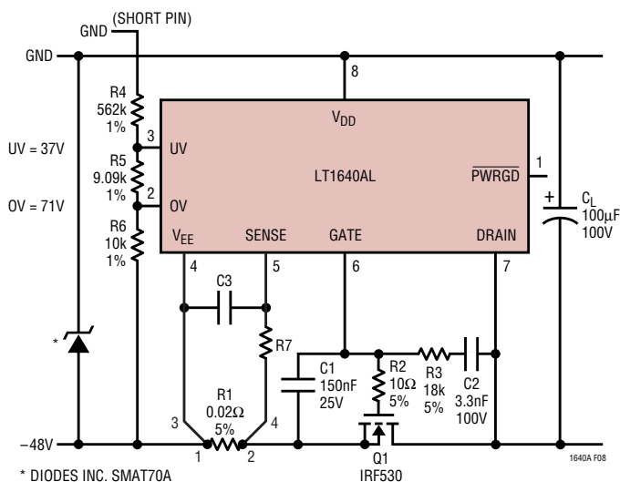
Figure 8. Extending the Short-Circuit Protection Delay
