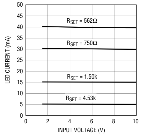
LED Current
