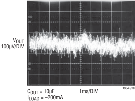
LT1964-5, 10Hz to 100kHz Output Noise, C_{BYP} = 1000\text{pF}
