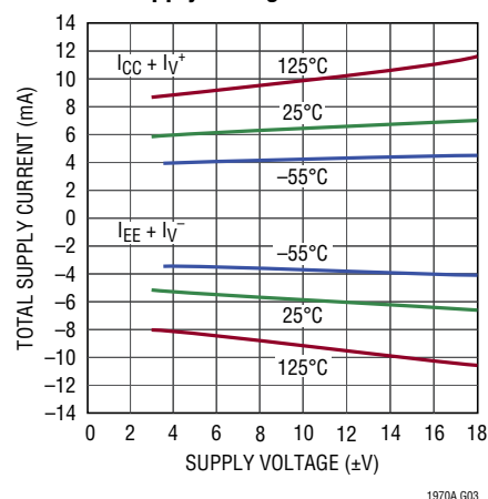
Total Supply Current vs Supply Voltage
