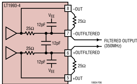
Figure 6. LT1993-4 Internal Filter Topology Modified for 2x Filter Bandwidth (2 External Resistors)
