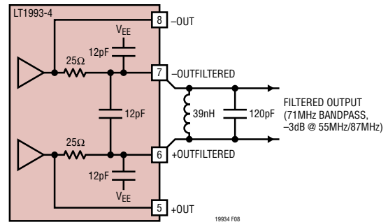
Figure 8. LT1993-4 Output Filter Topology Modified for Bandpass Filtering (1 External Inductor, 1 External Capacitor)
