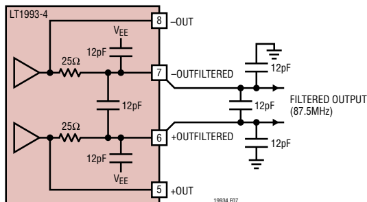
Figure 7. LT1993-4 Internal Filter Topology Modified for 1/2x Filter Bandwidth (3 External Capacitors)
