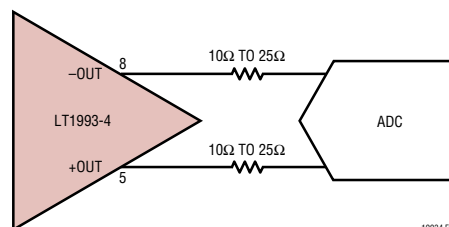
Figure 4. Adding Small Series R at LT1993-4 Output
