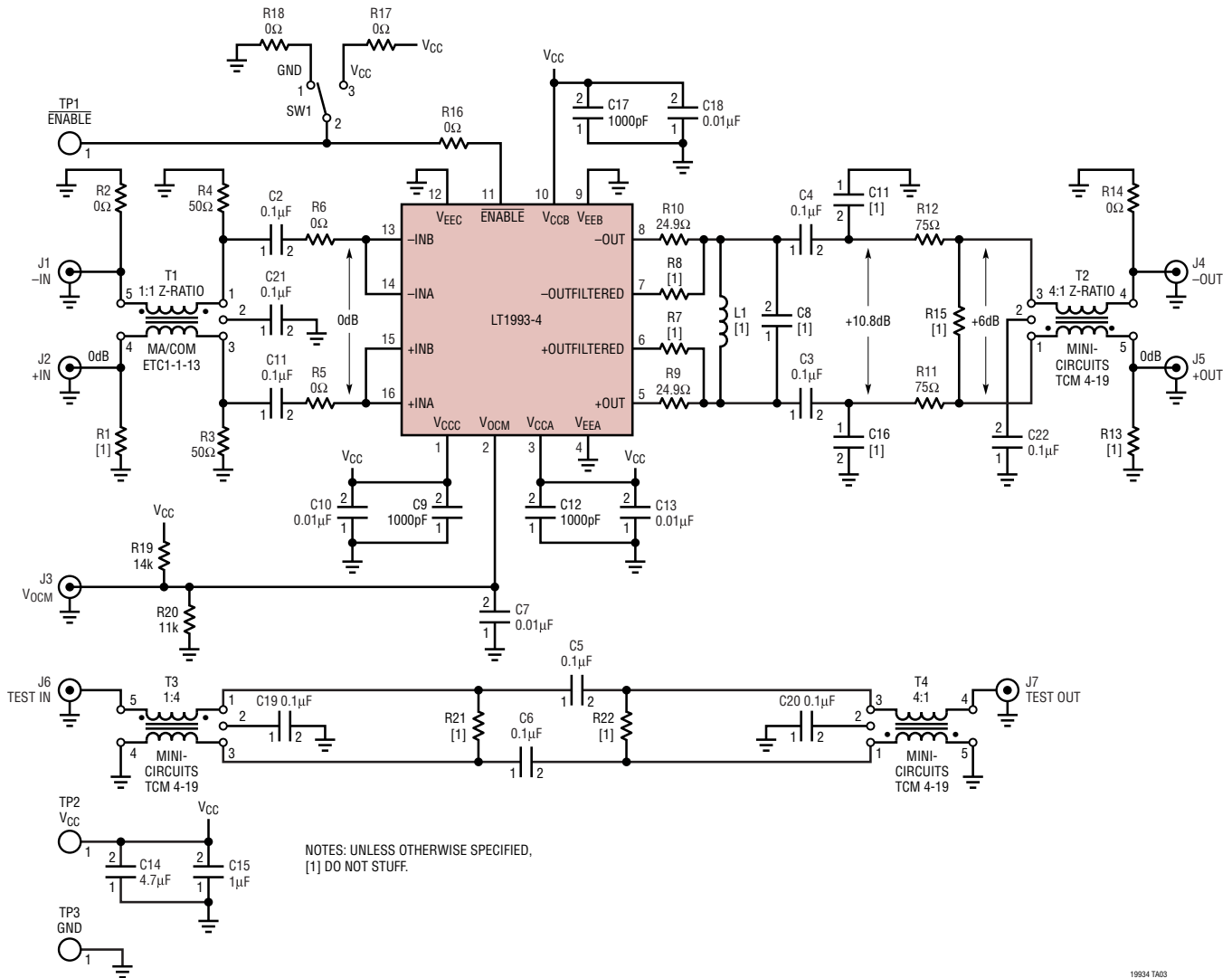
Demo Circuit DC800A Schematic (AC Test Circuit)
