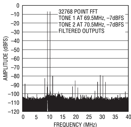
70MHz 2-Tone 32768 Point FFT LT1993-4 Driving LTC2249 14-Bit ADC
