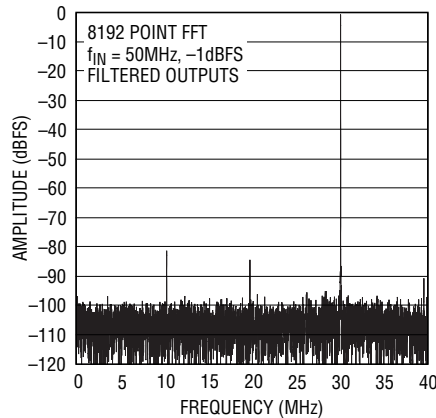
50MHz 8192 Point FFT, LT1993-4 Driving LTC2249 14-Bit ADC
