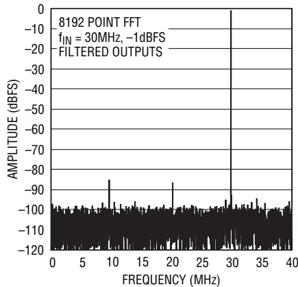
30MHz 8192 Point FFT, LT1993-4 Driving LTC2249 14-Bit ADC
