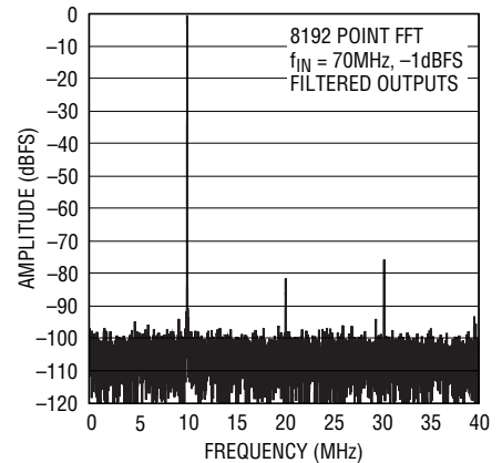
70MHz 8192 Point FFT, LT1993-4 Driving LTC2249 14-Bit ADC
