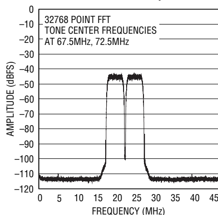
2-Tone WCDMA Waveform LT1993-4 Driving LTC2255 14-Bit ADC at 92.16Msps
