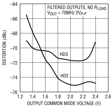
Distortion vs Output Common Mode Voltage, LT1993-4 Driving LTC2249 14-Bit ADC
