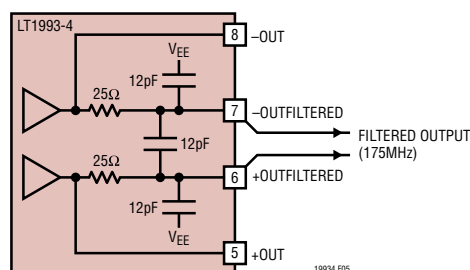
Figure 5. LT1993-4 Internal Filter Topology –3dB BW ≈175MHz
