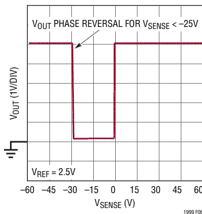
Figure 6. A Plot of the LT1999's Output Voltage vs V_{SENSE} ( V_{SENSE} = V_{+IN} - V_{-IN} ). In Applications Where the Sense Voltage Is Driven in Excess of -25V, the Output of the LT1999 Will Undergo Phase Reversal
