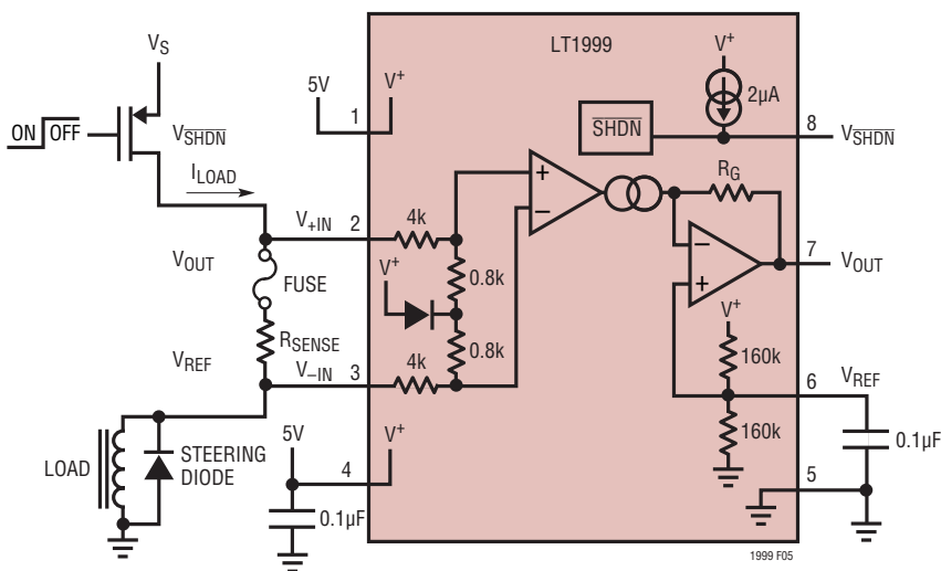
Figure 5. Using the LT1999 to Monitor a Fuse
