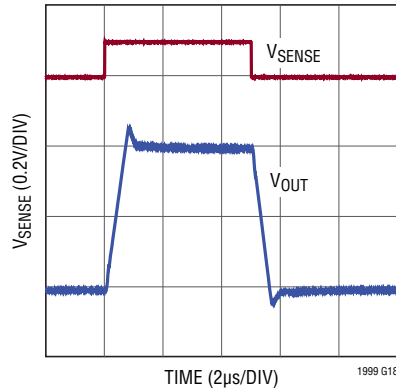
LT1999-20 Pulse Response
