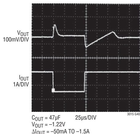
LT3015 Transient Response, C_{OUT} = 47\mu\text{F}
