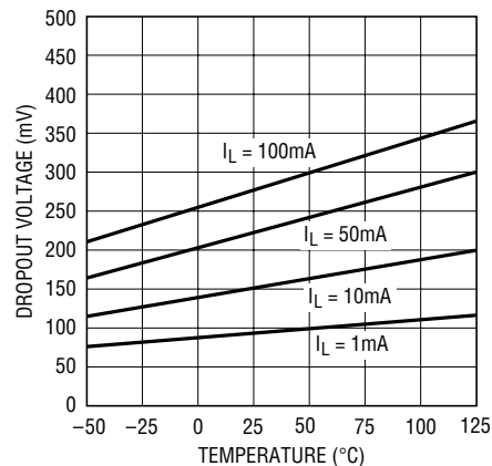
Output 2 Dropout Voltage
