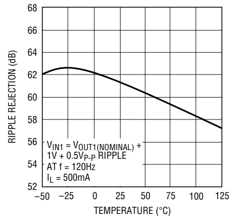
Output 1 Input Ripple Rejection
