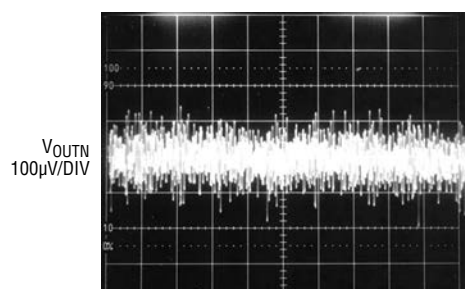
OUTN, 10Hz to 100kHz Output Noise, C_BYPN = 0.01µF
