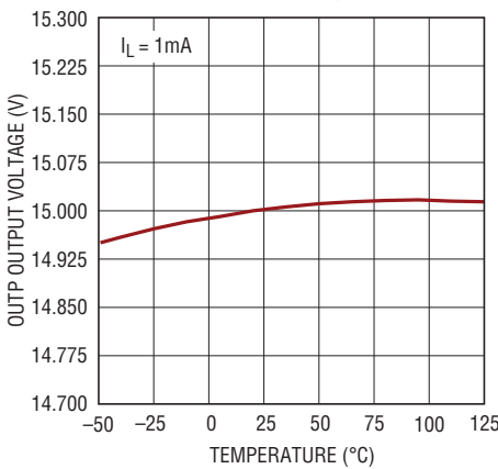
LT3032-15 OUTP Output Voltage
