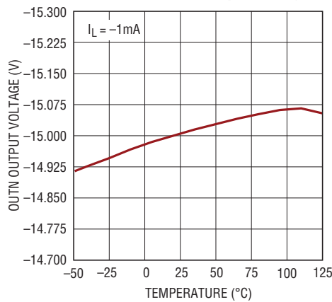
LT3032-15 OUTN Output Voltage
