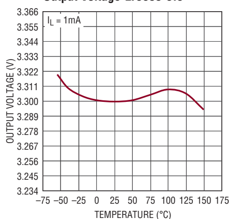
Output Voltage-LT3055-3.3
