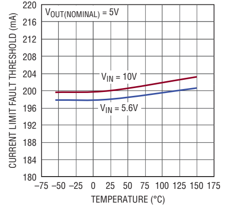
Precision Current Limit, R_{\text{IMAX}} = 1.5\text{k}\Omega
