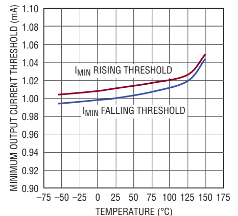
Minimum Output Current Threshold, R_{\text{IMIN}} = 1.2\text{M}\Omega
