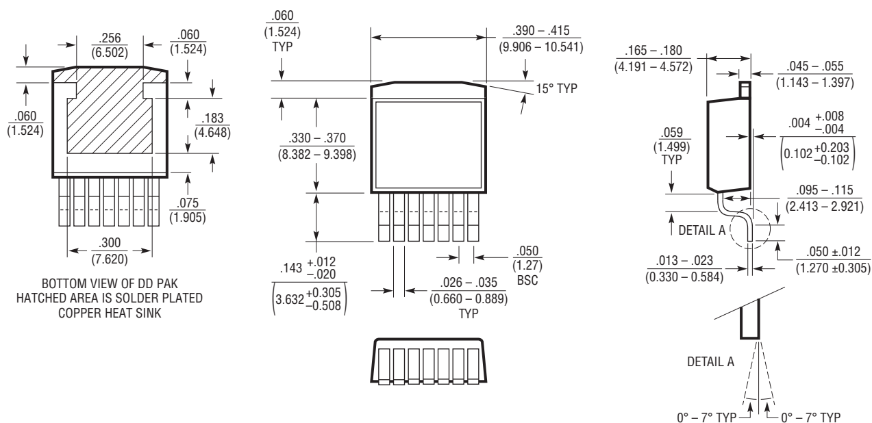
R Package 7-Lead Plastic DD Pak (Reference LTC DWG # 05-08-1462 Rev F)
