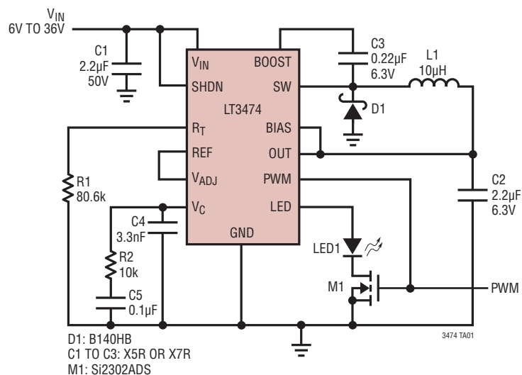
Step-Down 1A LED Driver with PWM Dimming
