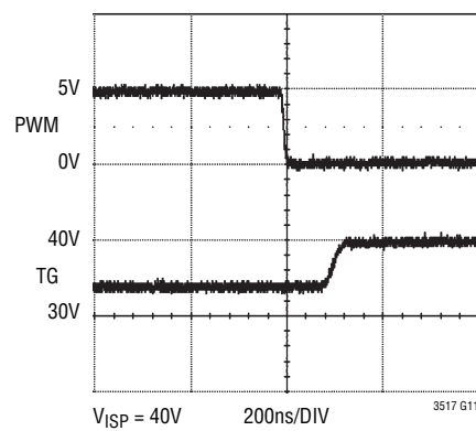
PMOS Turn-Off
