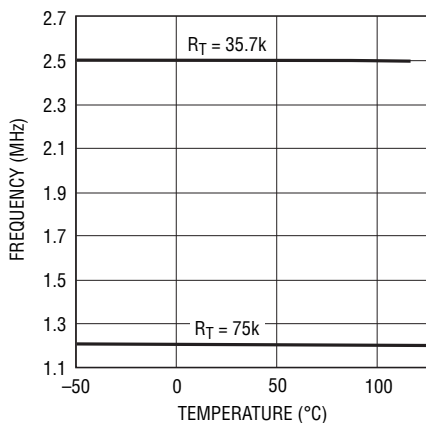
Oscillator Frequency
