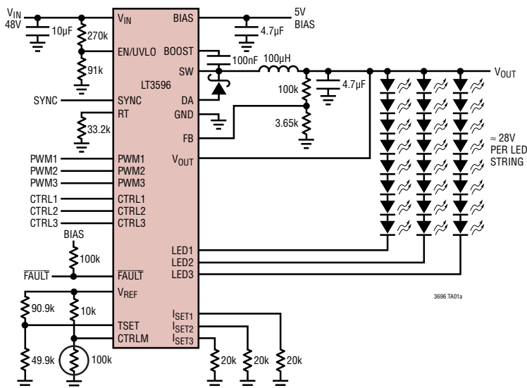
48V 1MHz Step-Down 8W, 100mA LED Driver (Eight White LEDs per Channel)
