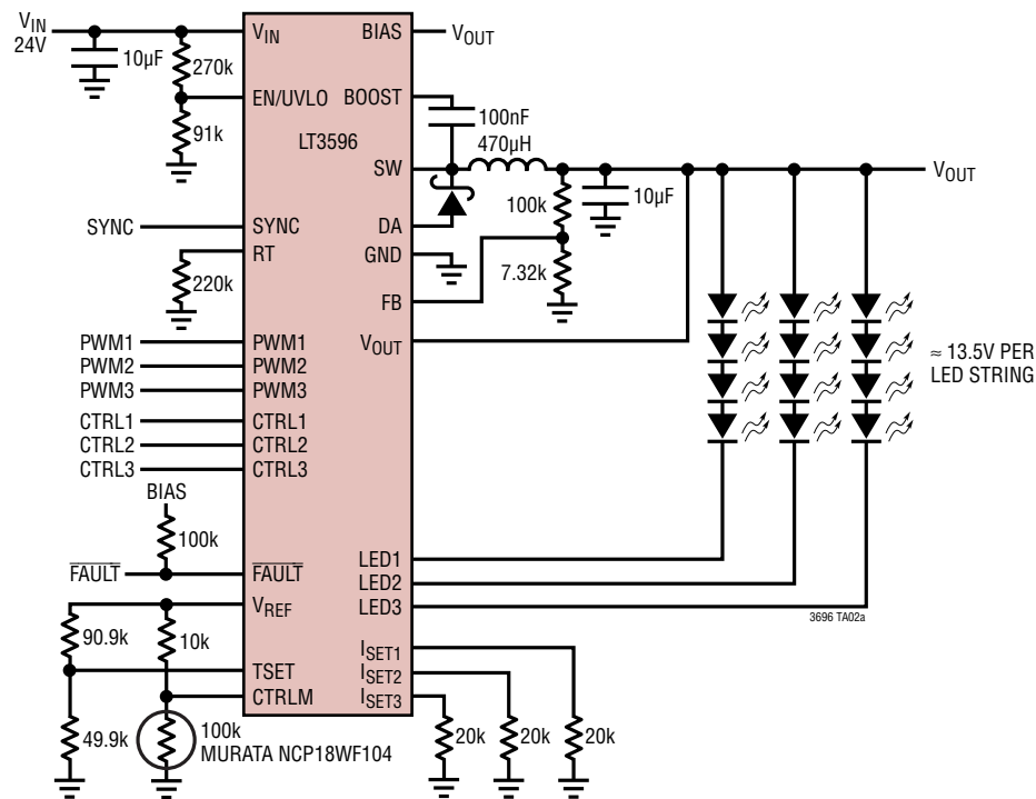
24V 200kHz Step-Down 4W, 100mA LED Driver
