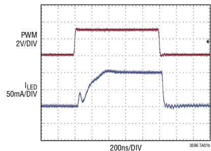
10,000:1 PWM Dimming at 100Hz
