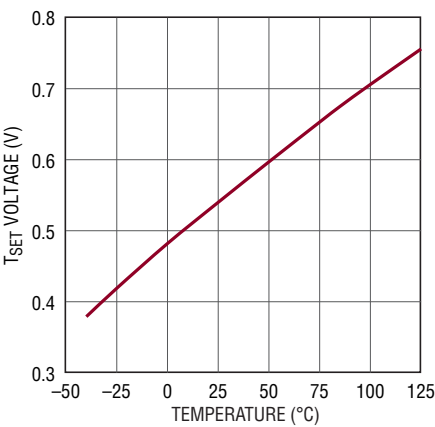
Figure 7. T SET Voltage for Temperature Derating
