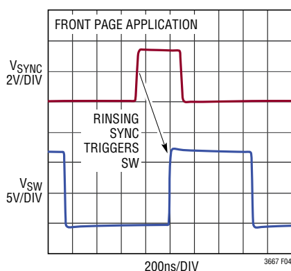
Figure 4. Synchronization Waveforms
