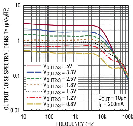
LD0s: Output Noise Spectral Density
