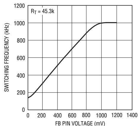
Frequency Foldback
