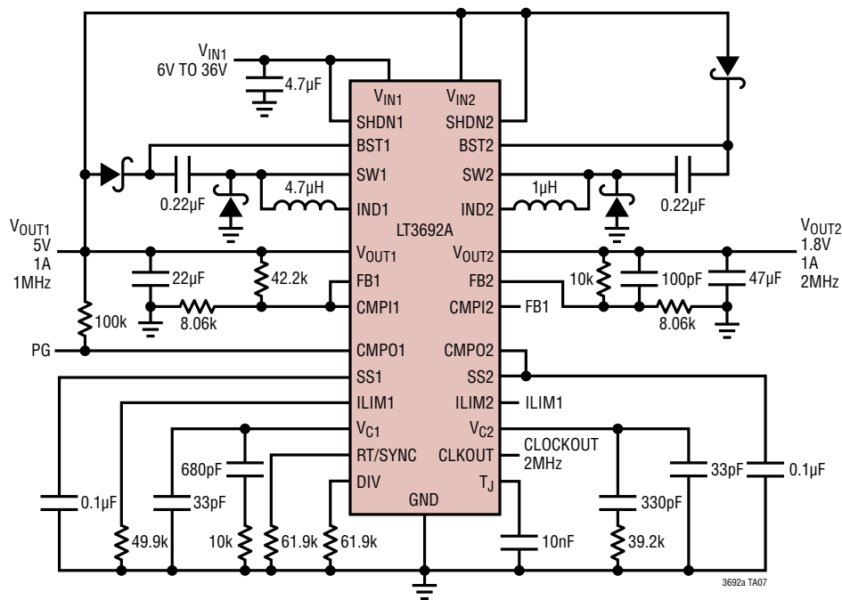
5V and 1.8V Dual 2-Stage Converter
