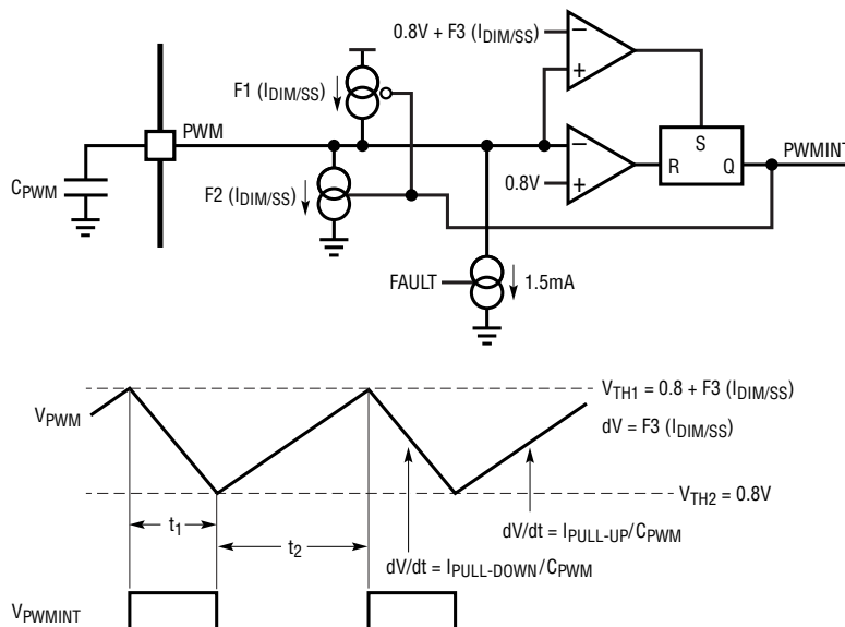
Figure 5. Internal PWM Oscillator Logic and Waveform
