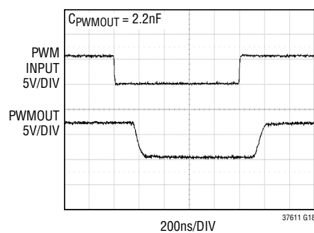
PWMOUT Waveform
