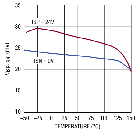
V ISP-ISN C/10 Threshold vs Temperature
