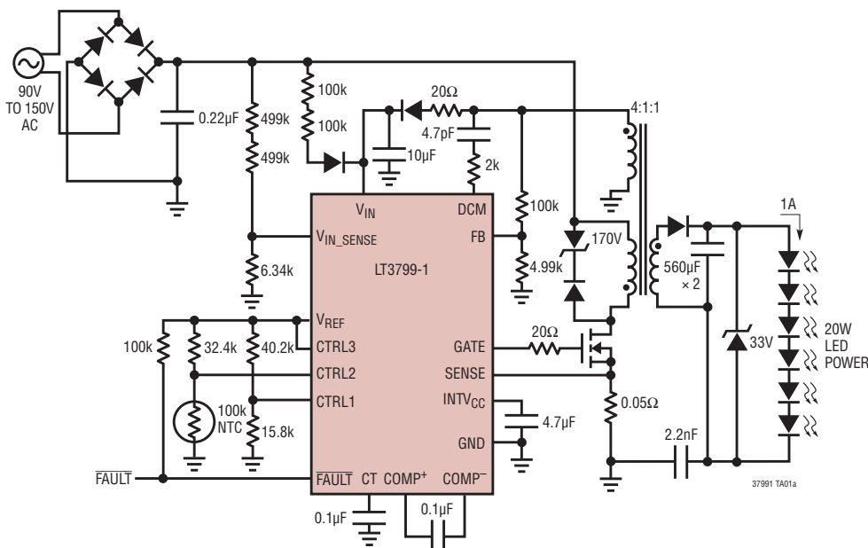
20W LED Driver
