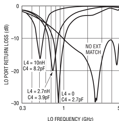
Figure 6. LO Input Return Loss
