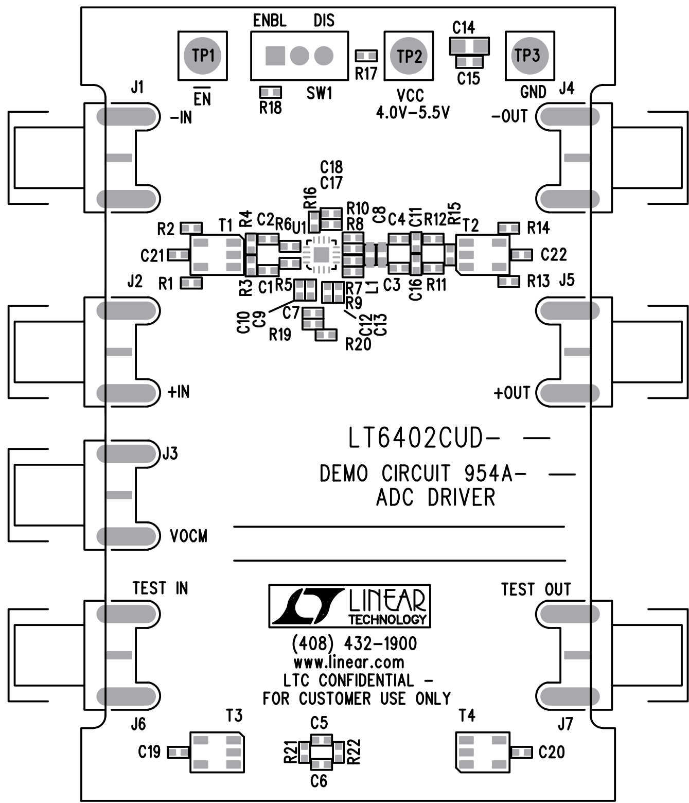
Top Silkscreen
