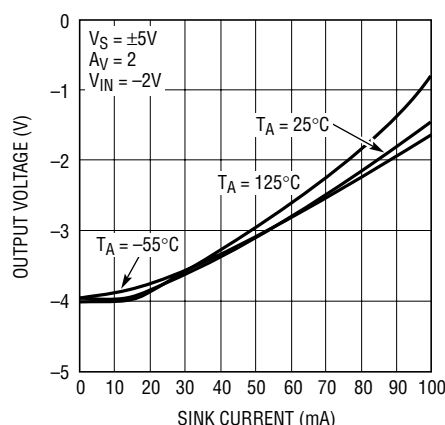
Output Voltage Swing vs I LOAD (Output Low)
