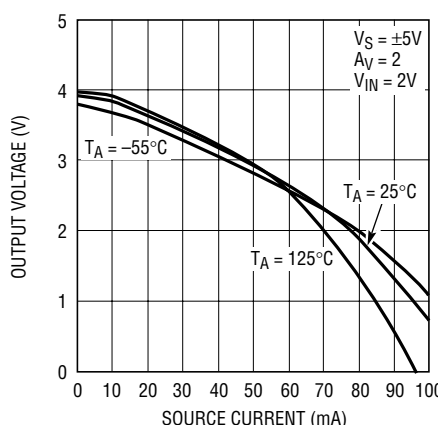
Output Voltage Swing vs I LOAD (Output High)
