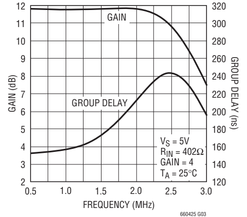
Passband Gain and Group Delay
