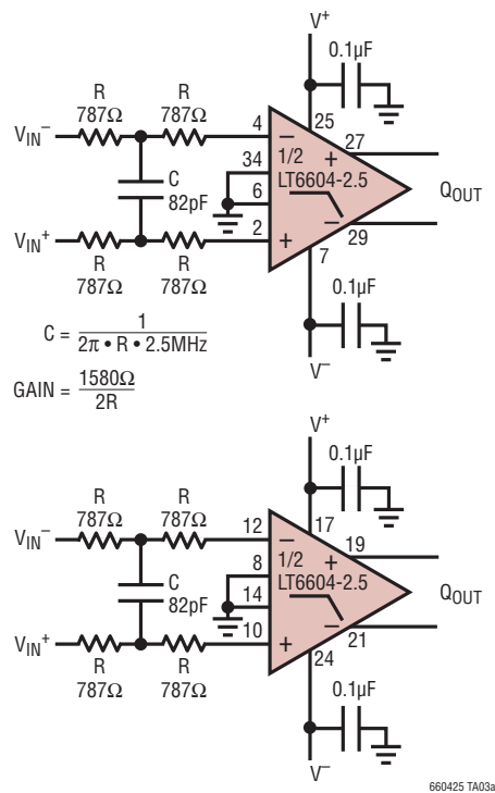
Dual, Matched 5th Order, 2.5MHz Lowpass Filter, Gain = 1
