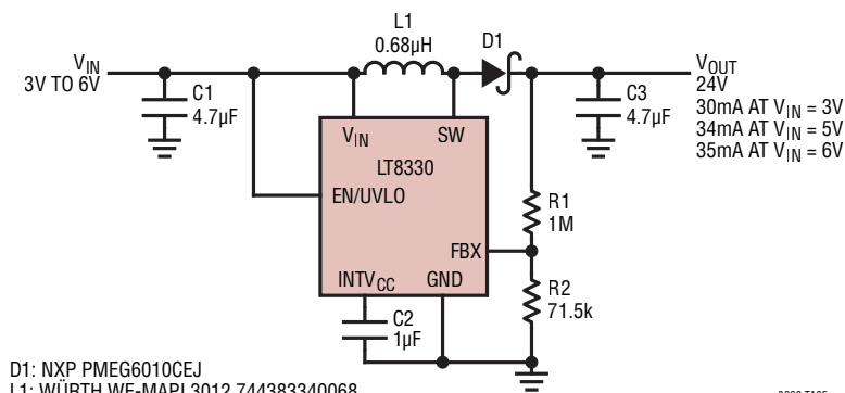
3V to 6V Input, 24V Boost Converter
