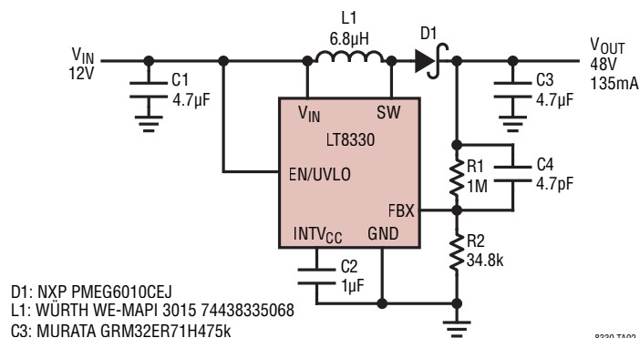
48V Boost Converter
