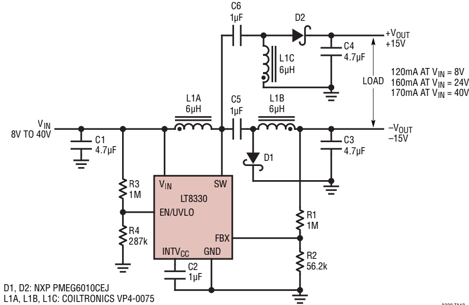
8V to 40V Input, \pm 15V Converter
