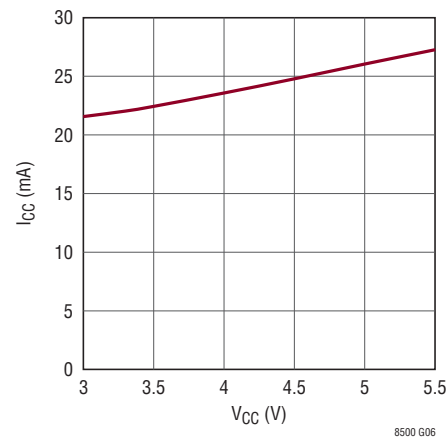
I_{CC} vs V_{CC} , SCKI = 50MHz, SDI = 25MHz, PWMCK = 25MHz
