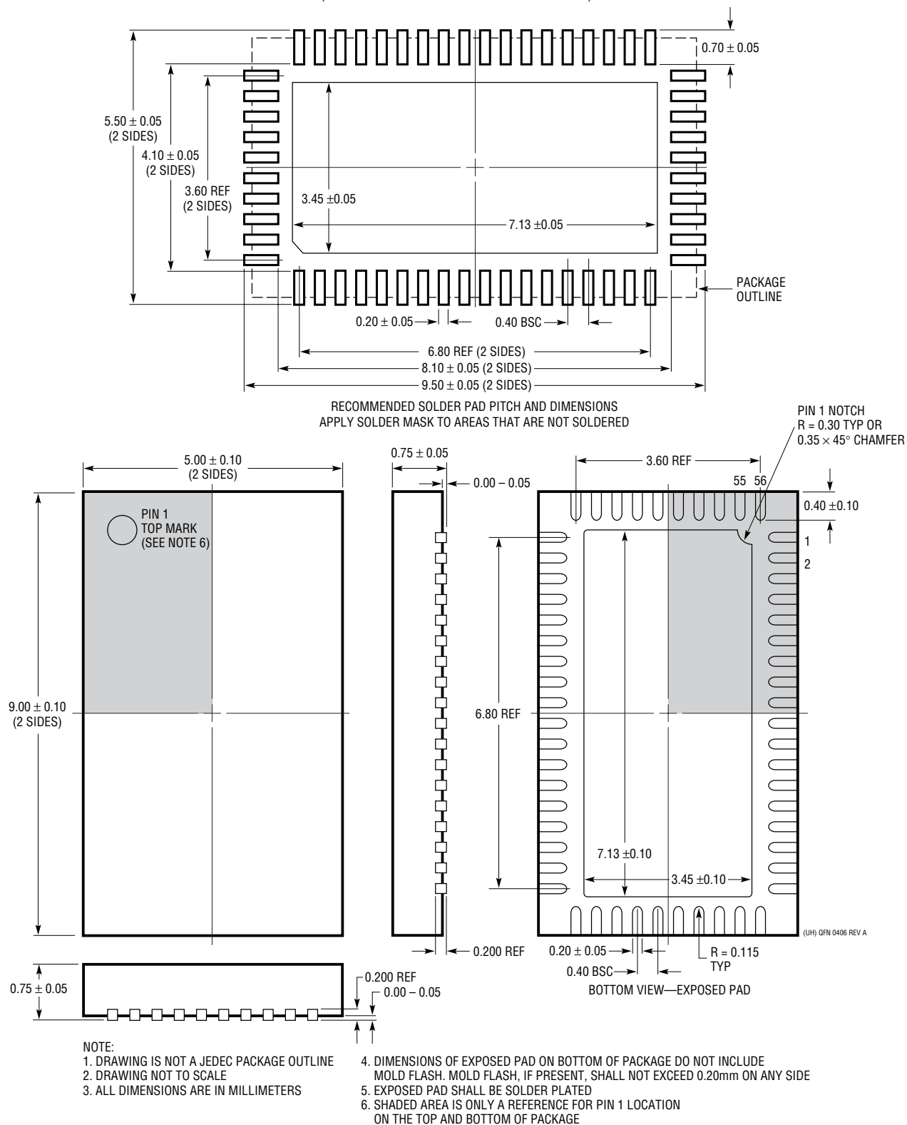
UHH Package 56-Lead (5mm × 9mm) Plastic QFN (Reference LTC DWG # 05-08-1727 Rev A)
